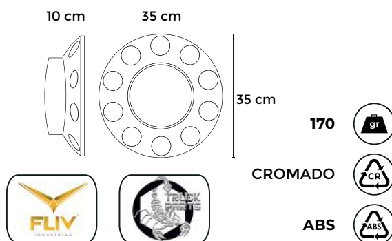
REF: 5002R TAPA RIN ESFERA
