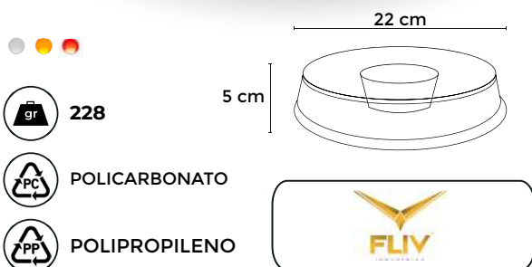
REF: VEC57- L570 VASO EXTERNO POLICARBONATO
